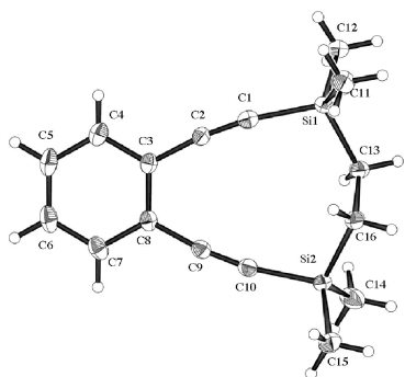
Figure 1. ORTEP drawing of 5a (50% probability for thermal ellipsoids). Selected bond lengths [Å] and angles [deg]: Si1–C1 1.847(4), C1–C2 1.210(5), C2–C3 1.432(5), C3–C8 1.399(5), Si1–C1–C2 169.1(3), C1–C2–C3 172.6(4), C2–C3–C8 118.3(3), C1···C8 nonbonded distance, 3.63 Å.
